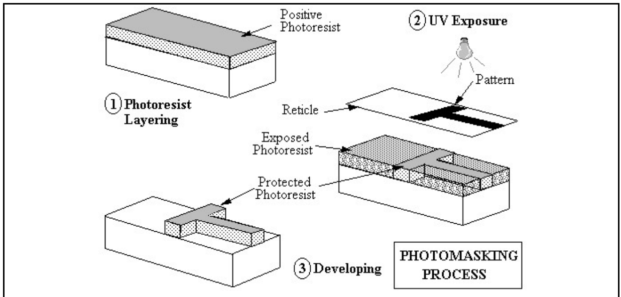
Figure 3. Photomasking Process
