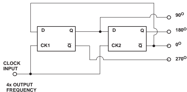
Figure 9. Dual Flip-Flop Quadrature Synthesis
