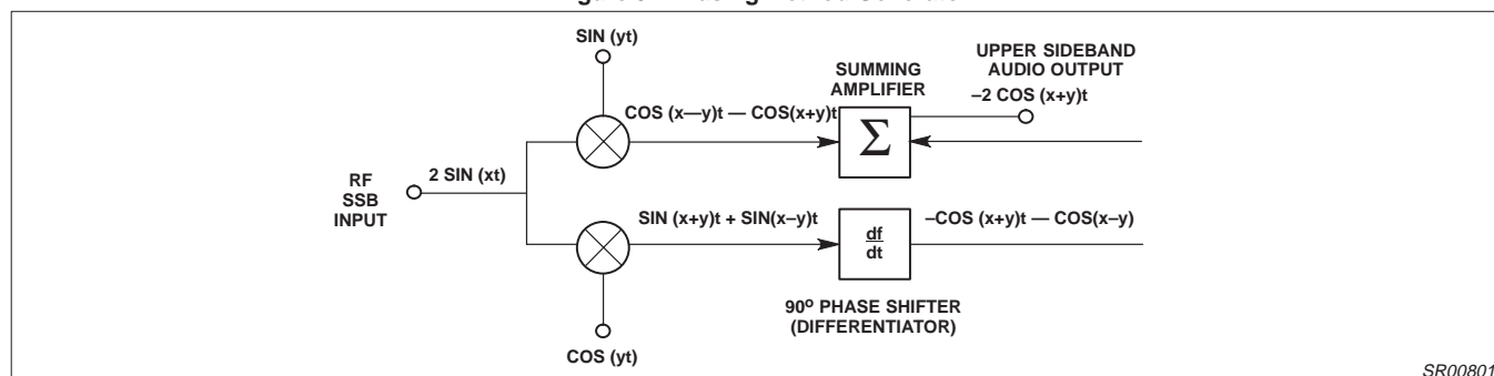
Figure 6. Phasing Method Detector with Simplified Mathematical Model
